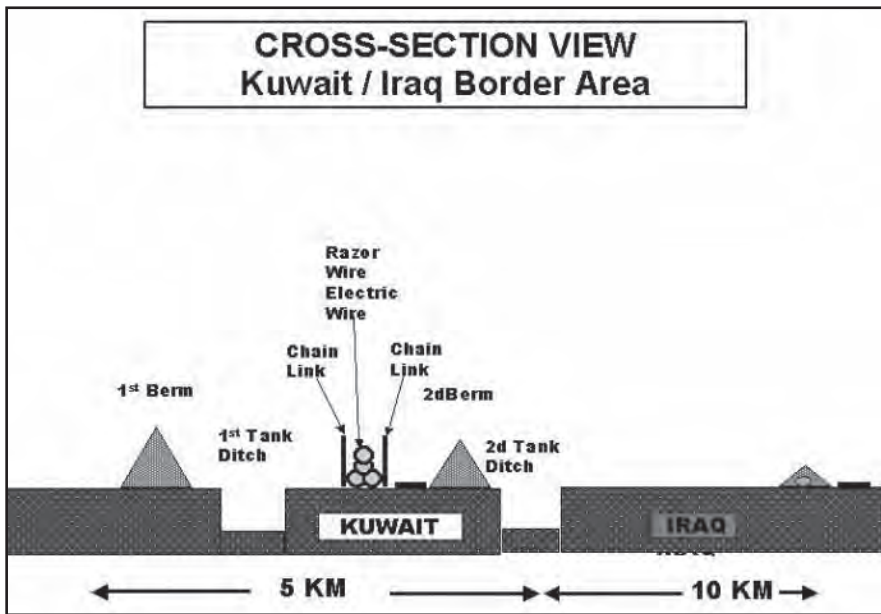
Figure 48. Kuwait-Iraq berm cross-section
